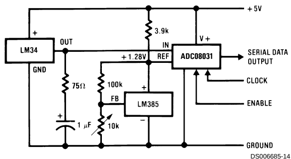
Temperature-to-Digital Converter (Serial Output, +128°F Full Scale)
