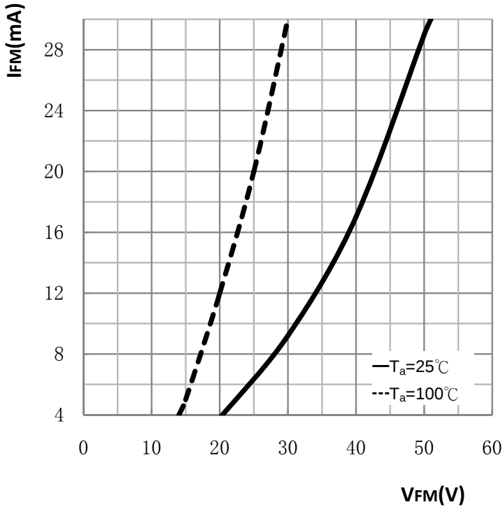
Figure 1. Forward characteristics
