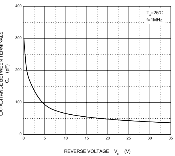
Capacitance Characteristics
