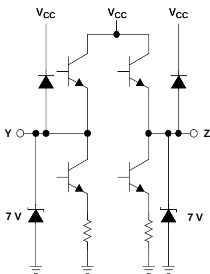
OUTPUT LVDS16/17
