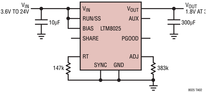
1.8V Step-Down Converter
