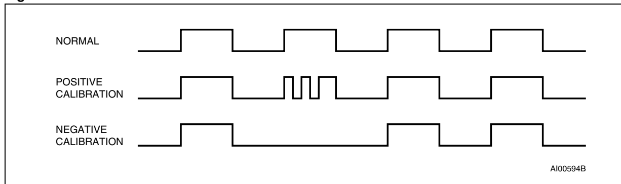
Figure 12. Clock calibration
