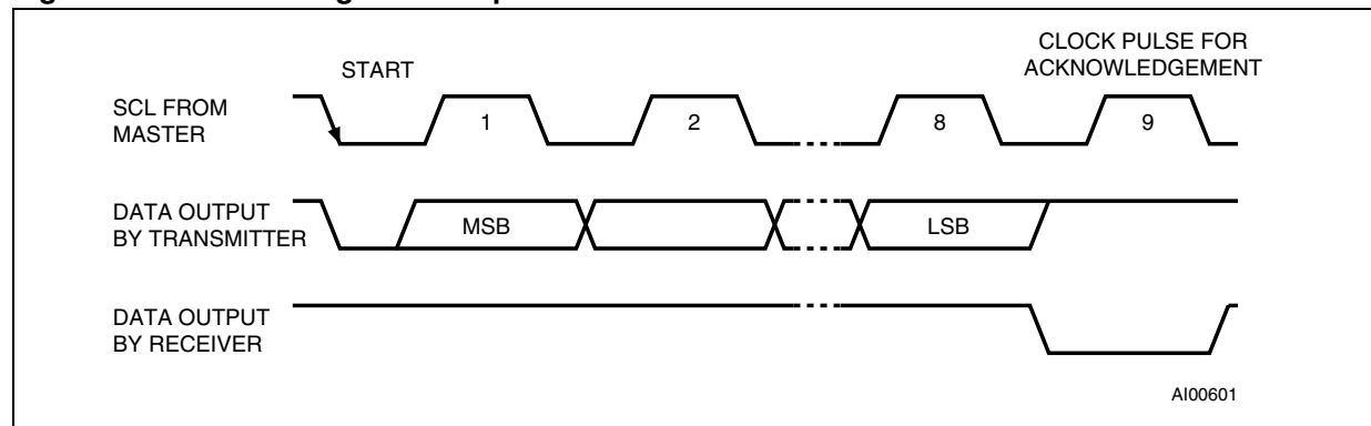
Figure 5. Acknowledgement sequence
