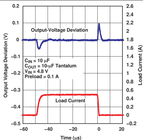
图 6-7. TLV1117-33 Load Transient Response
