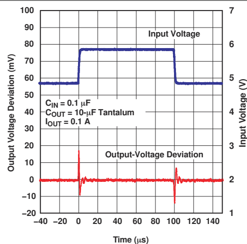
图 6-8. TLV1117-33 Line Transient Response
