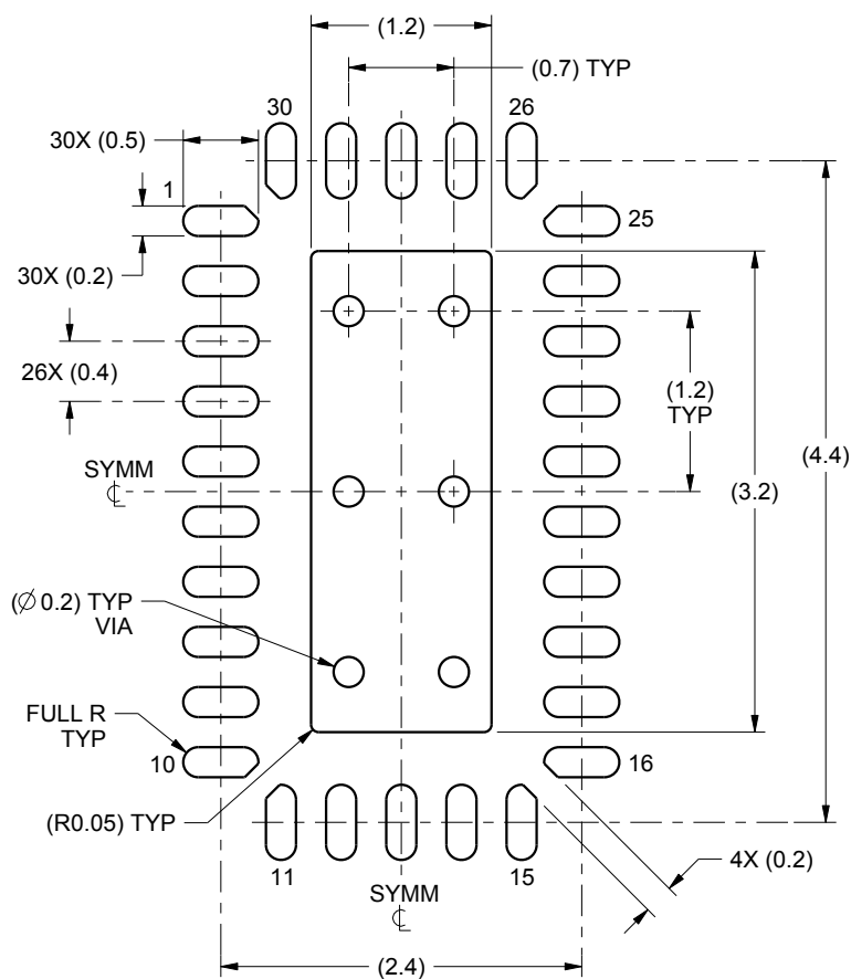
LAND PATTERN EXAMPLE SCALE:18X
