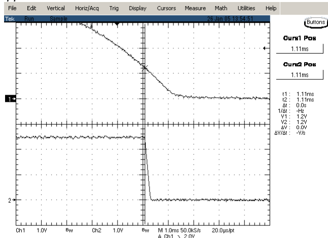
Figure 18: Remote turn off delay time at 24vin, 2.5V/3A out
