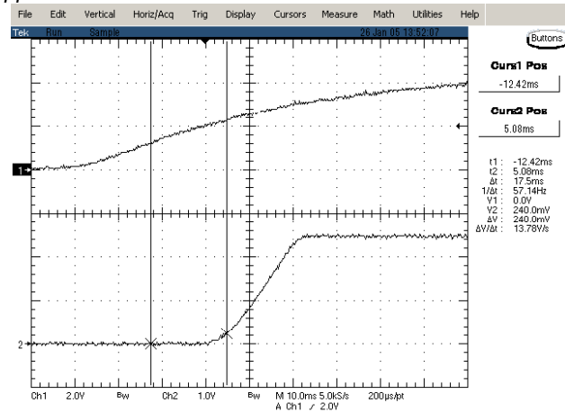
Figure 17: Remote turn on delay time at 24vin, 2.5V/3A out
