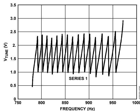
Figure 17. VCO Bands
