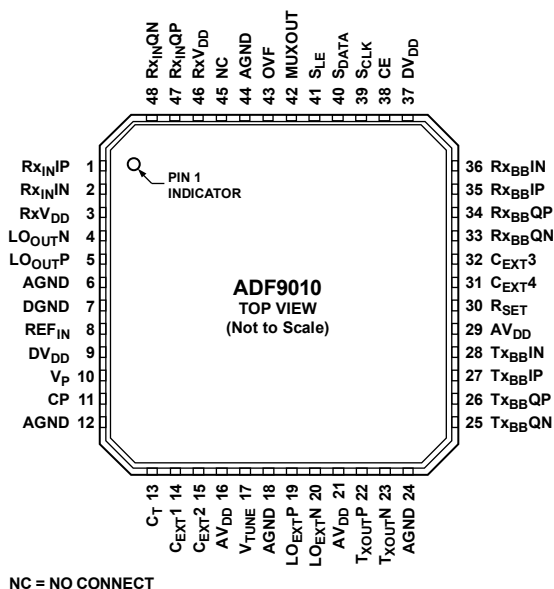
Figure 3. Pin Configuration
