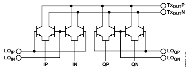
Figure 20. Tx Section
