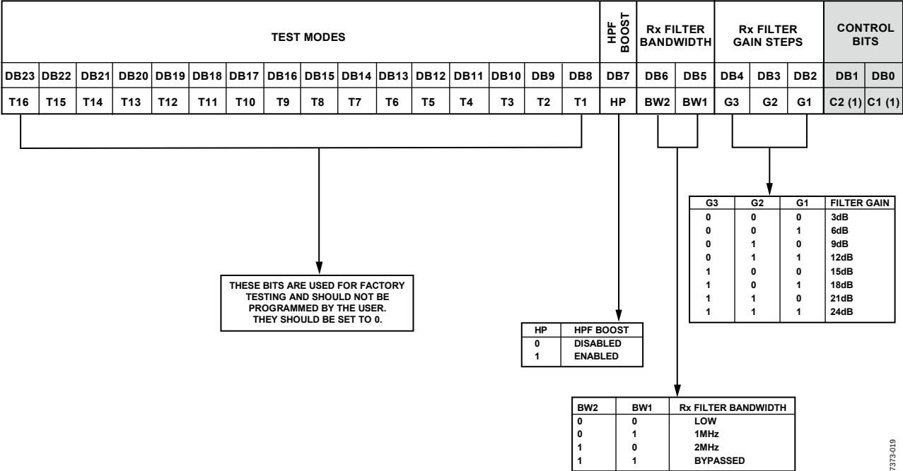
Figure 26. Rx Latch
