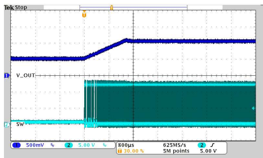
50% PreBias Start No Load
