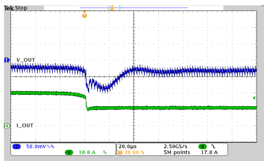
Load Release 20A to 10A
