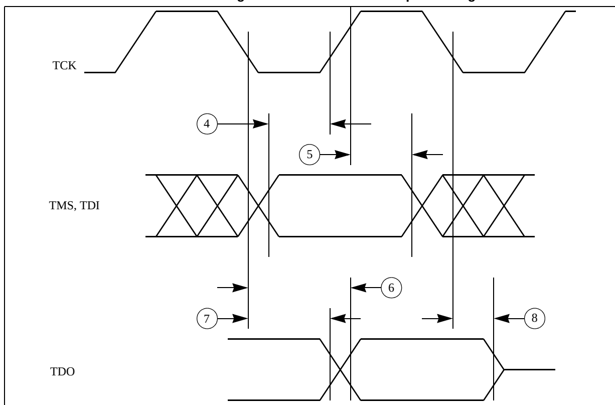
Figure 24. JTAG test access port timing
