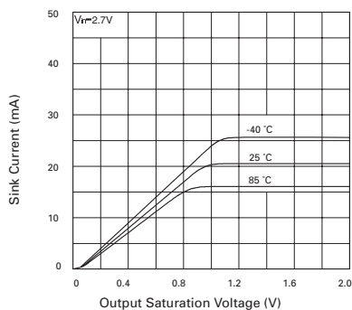
Output Saturation Voltage vs. Sink Current
