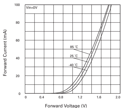
Clamp Diode Forward Current vs. Voltage
