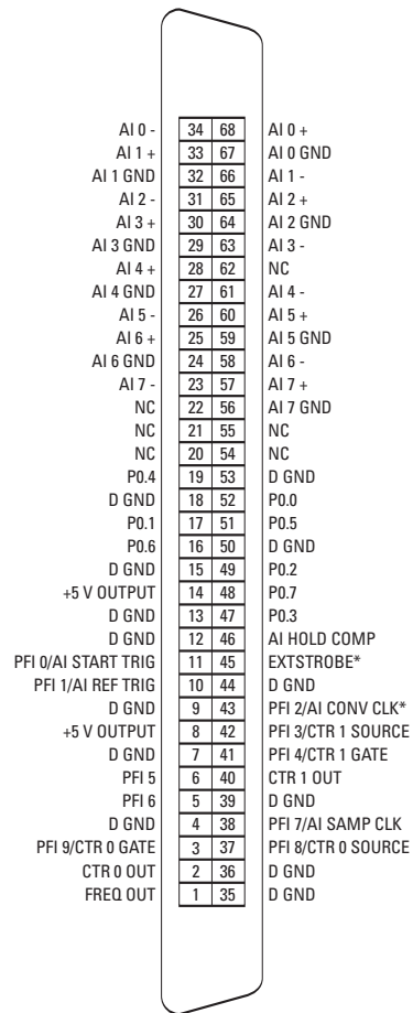
Figure 3. I/O Connector
