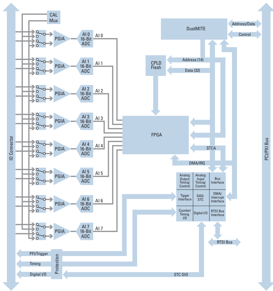
Figure 2. Block Diagram
