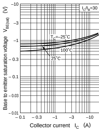
V_{BE(\text{sat})} - I_C
