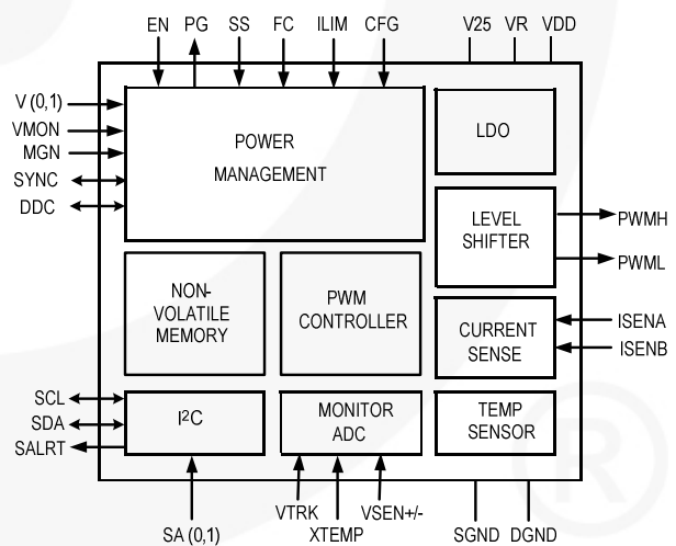
Figure 1. Block Diagram
