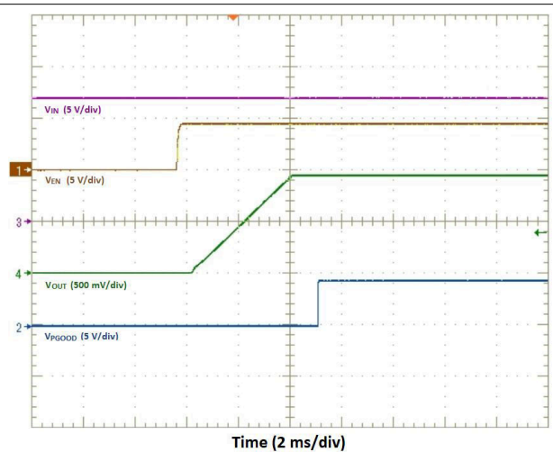
Figure 8-3. Start-Up Waveforms
