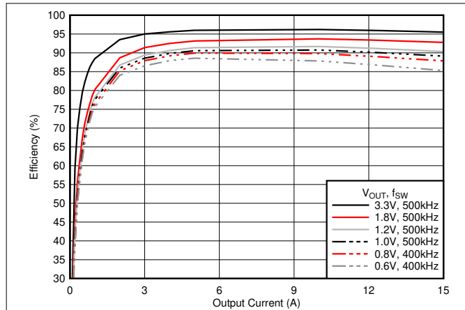
Figure 6-7. Efficiency vs Output Current
