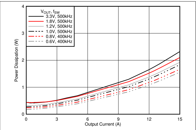
Figure 6-8. Power Dissipation vs Output Current
