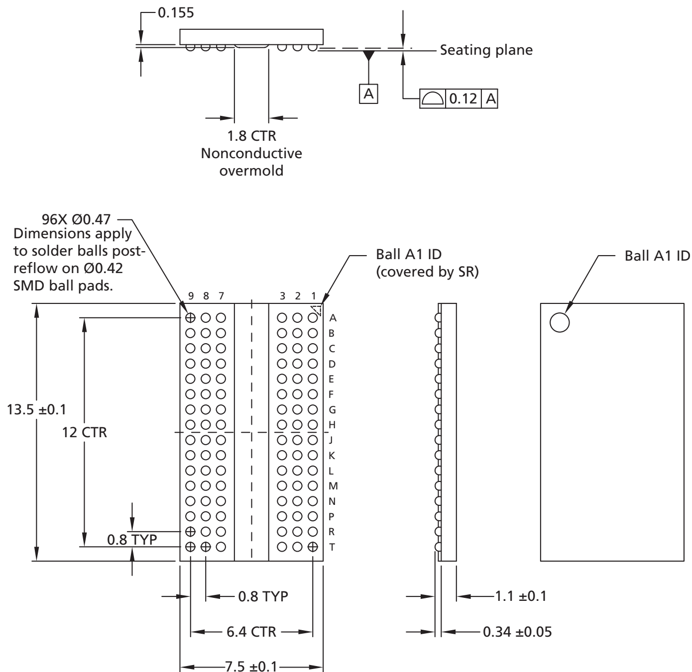
Figure 12: 96-Ball FBGA – x16 (LY)
