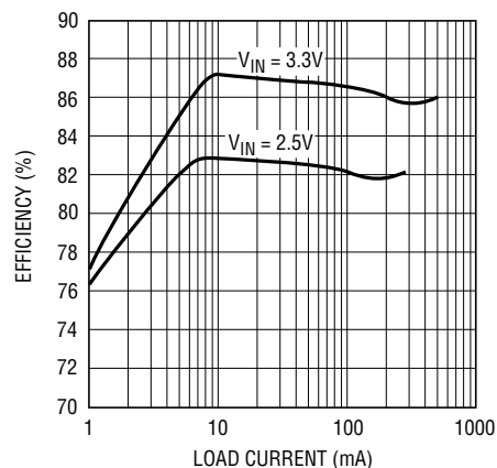
5V Output Efficiency
