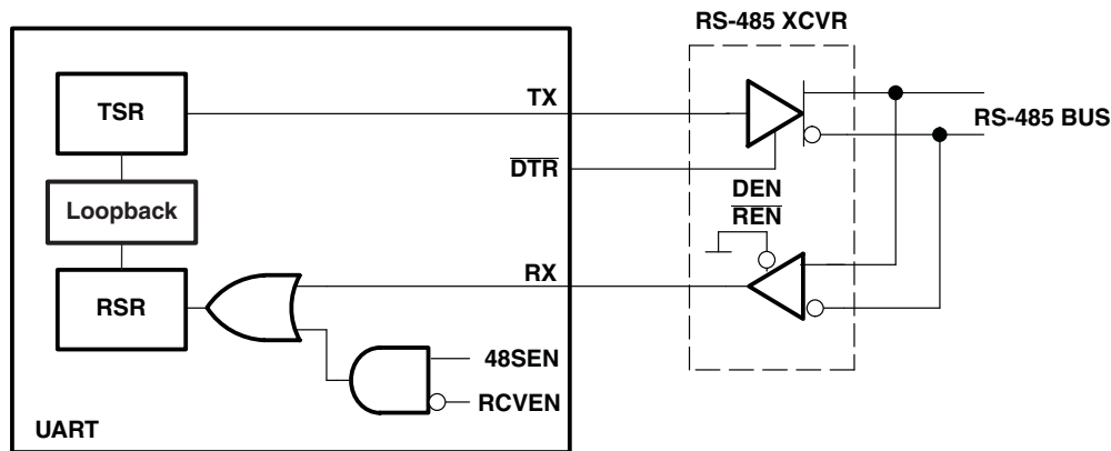
Figure 25. RS-485 Application Example 2
