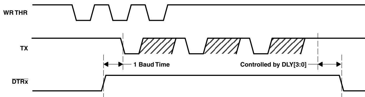
Figure 23. \overline{\text{DTRx}} and Transmit Data Relationship
