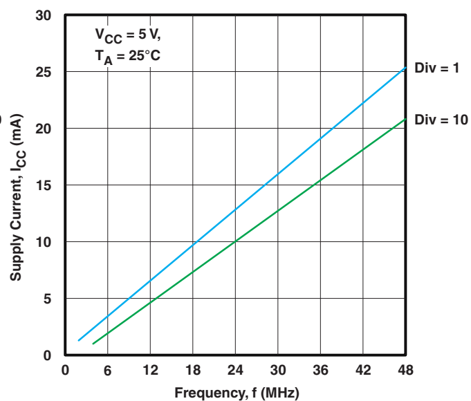
Figure 12. Supply Current vs Frequency ( V_{CC} = 5\text{ V} )
