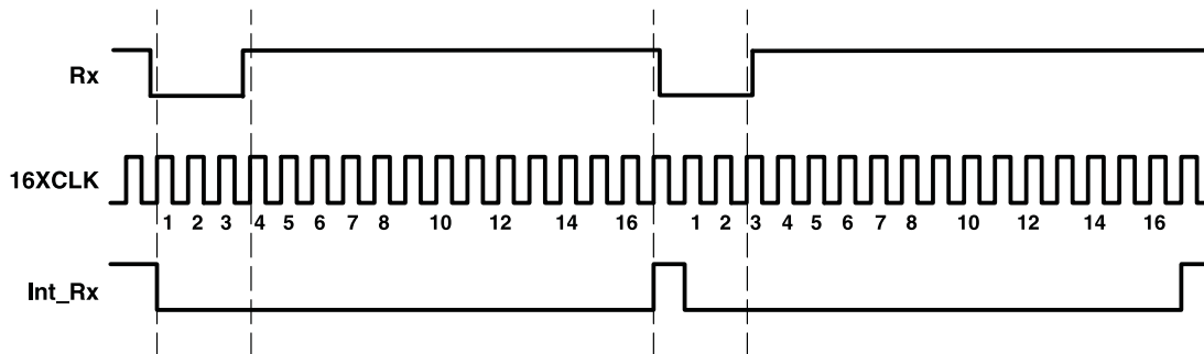
Figure 31. Timing Causing 1-Clock-Wide Pulse Between Consecutive Ones
