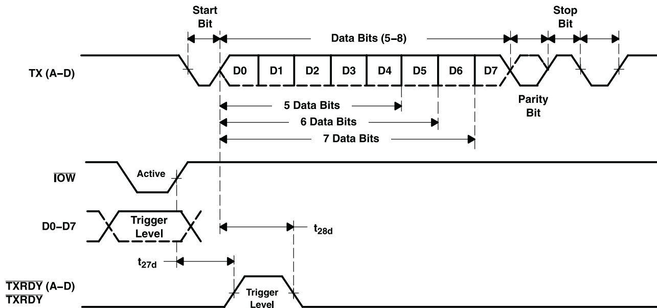
Figure 21. Transmit Timing in FIFO Mode
