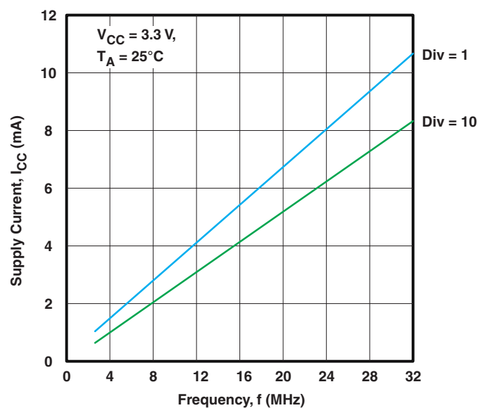
Figure 11. Supply Current vs Frequency ( V_{CC} = 3.3\text{ V} )
