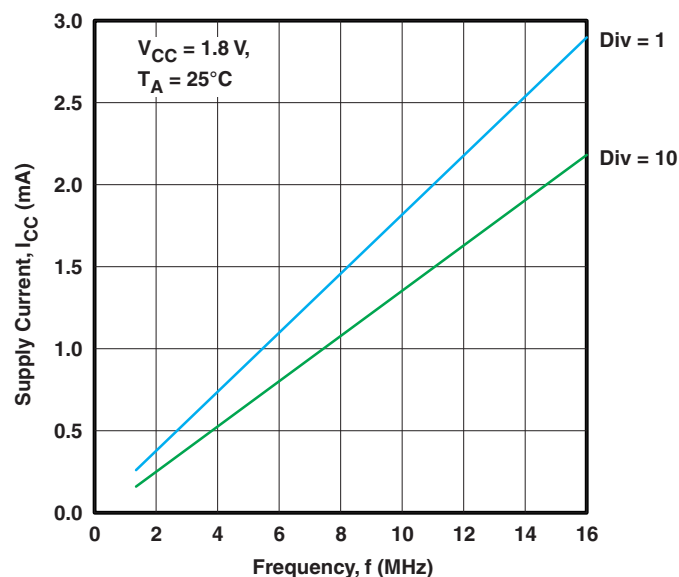
Figure 9. Supply Current vs Frequency ( V_{CC} = 1.8\text{ V} )
