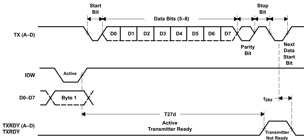
Figure 20. Transmit Ready Timing in None FIFO Mode
