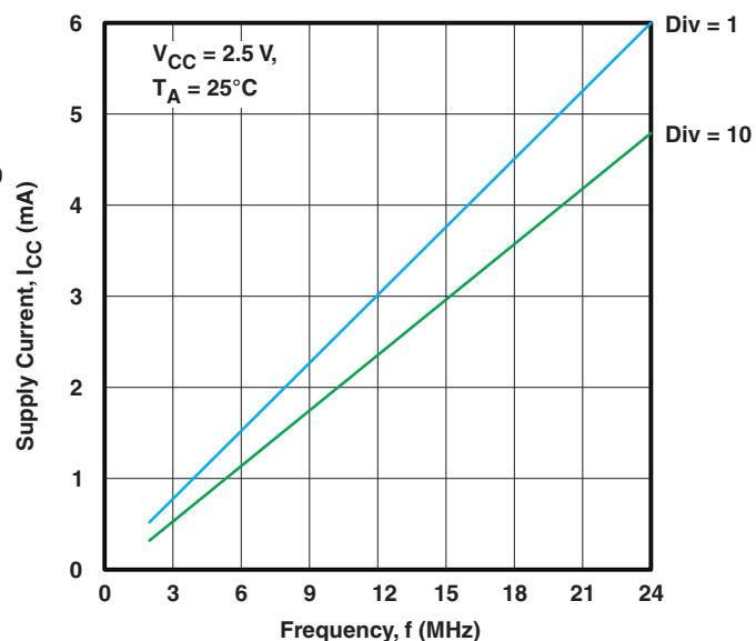
Figure 10. Supply Current vs Frequency ( V_{CC} = 2.5\text{ V} )
