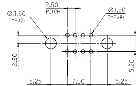
RECOMMENDED P.C.B HOLE DIM.(MOUNT SIDE)
