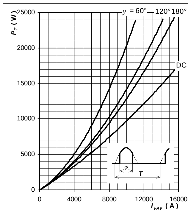
Fig. 6 Forward power loss vs. average forward current, sine wave waveform, f = 50 \text{ Hz} , T = 1/f
