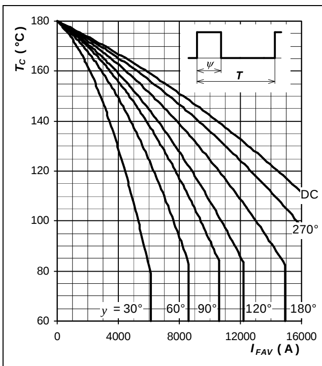
Fig. 9 Max. case temperature vs. aver. forward current, square waveform, f = 50 Hz, T = 1/f
