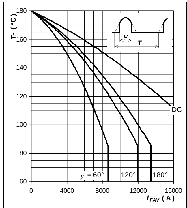
Fig. 8 Forward power loss vs. average forward current, sine waveform, f = 50 Hz, T = 1/f
