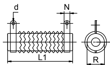
Non-Inductive Power Resistors (DQBN) N - No mount Dimensions
