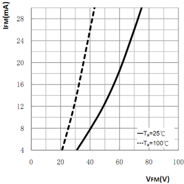
Forward Characteristics
