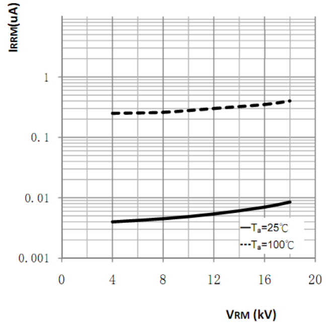
Reverse Characteristics
