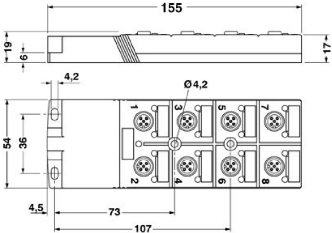
Dimensioned drawing
