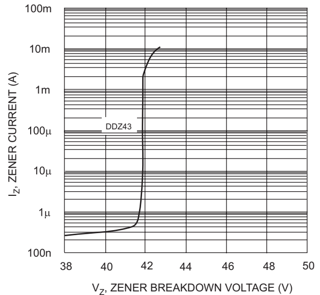
Fig. 9 Typical Reverse Characteristics, DDZ43
