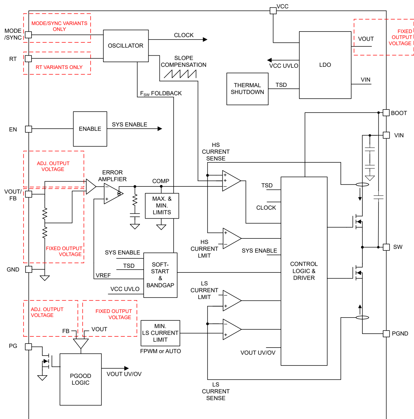
Figure 8-1. LMQ664x0 Functional Block Diagram
