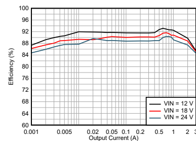
Efficiency: V_{OUT} = 3.3 \text{ V} (Fixed), 2.2 MHz
