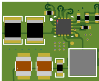
Typical Solution Size (16.5 mm \times 13.5 mm)
