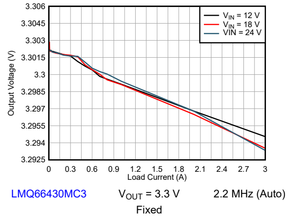
Figure 9-6. Line and Load Regulation
