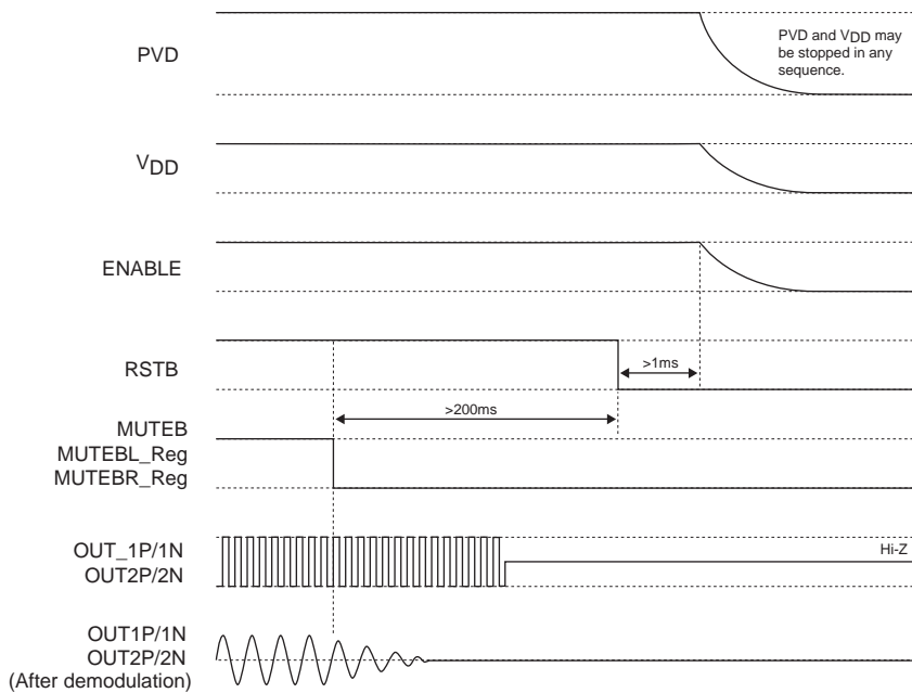
Figure 3.2 Stop sequence
