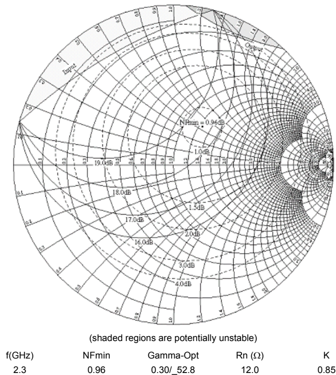
Figure 22. Constant Noise Figure and Gain Circles. 2400 MHz, Rbias = 1.2 kΩ
