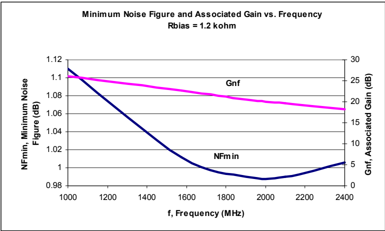
Figure 6. Minimum Noise Figure and Associated Gain vs. Frequency ( R_{bias} = 1.2\text{ k}\Omega )
