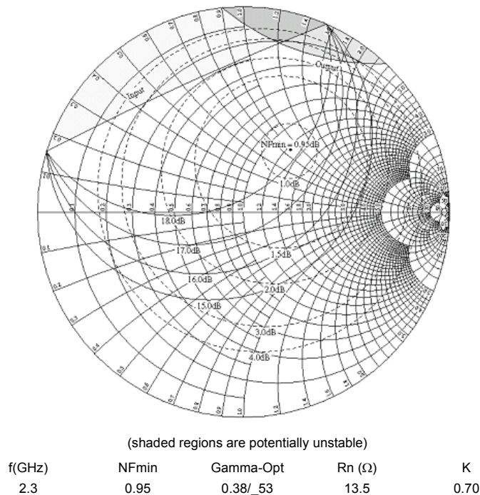
Figure 23. Constant Noise Figure and Gain Circles. 2400 MHz, Rbias = 2 kΩ
