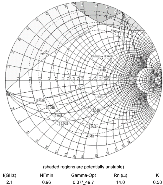
Figure 21. Constant Noise Figure and Gain Circles. 2140 MHz, Rbias =1.2 kΩ
