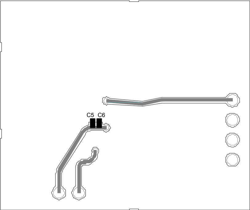
Figure 15. Back Side
