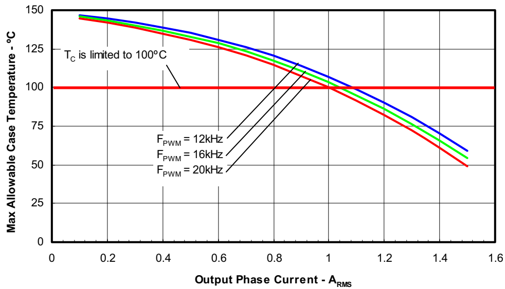
Figure 9. Maximum Allowable Case Temperature vs. Output RMS Current per Phase Sinusoidal Modulation, V^+ = 360\text{V} , T_J = 150^\circ\text{C} , Modulation Depth=0.8, PF=0.6
