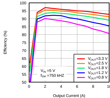
Figure 11. Efficiency
