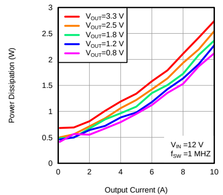
Figure 6. Power Dissipation
