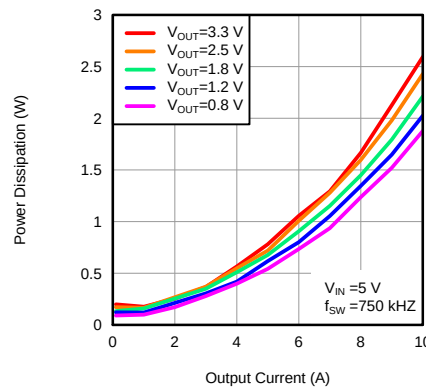
Figure 14. Power Dissipation
