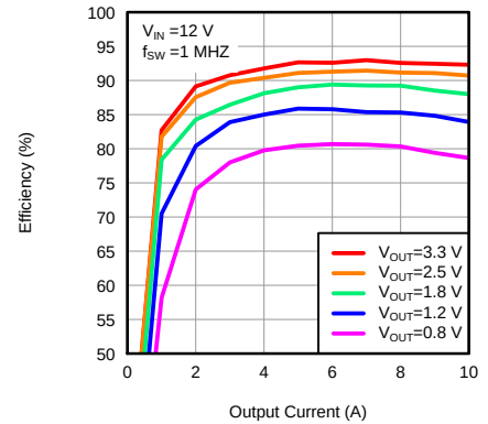
Figure 3. Efficiency
