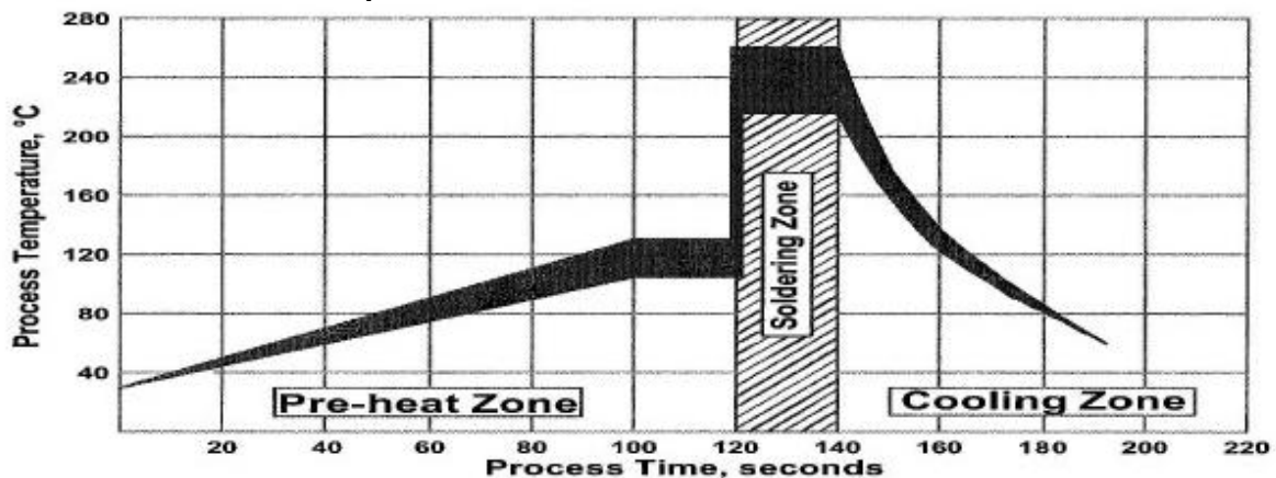
Temperature Profile for Water-based Flux
