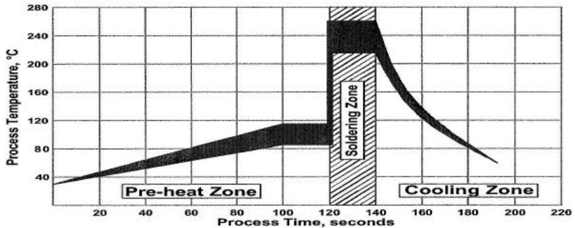
Temperature Profile for Alcohol-based Flux
