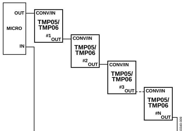
Figure 24. Daisy-Chain Structure
