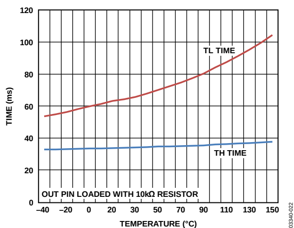
Figure 8. T H and T L Times vs. Temperature
