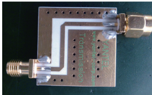
Transmission Board
