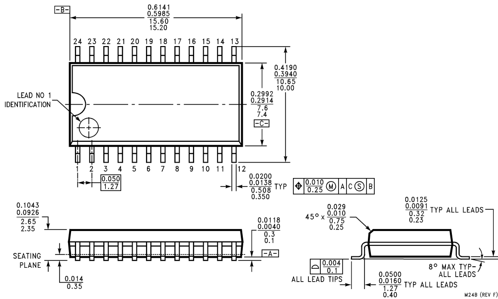
Order Number ADC10062CIWM NS Package Number M24B
