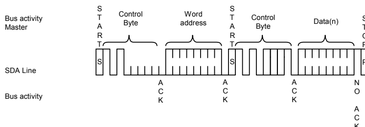
Figure 7-2. Random read
