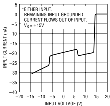
Input Characteristics*
