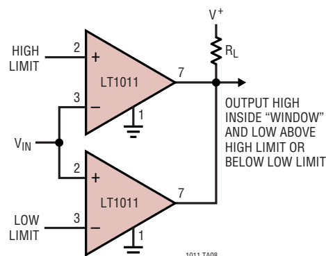
Window Detector
