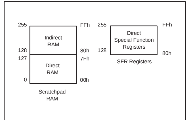
Figure 22. Register Map
