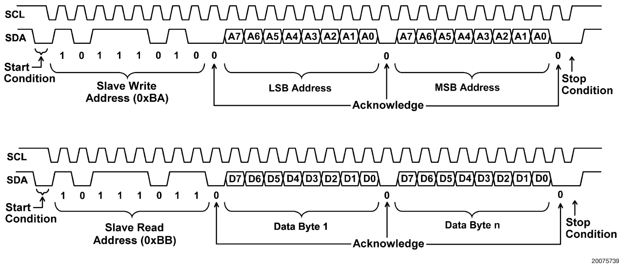
FIGURE 24. I²C Compatible Read Sequence
