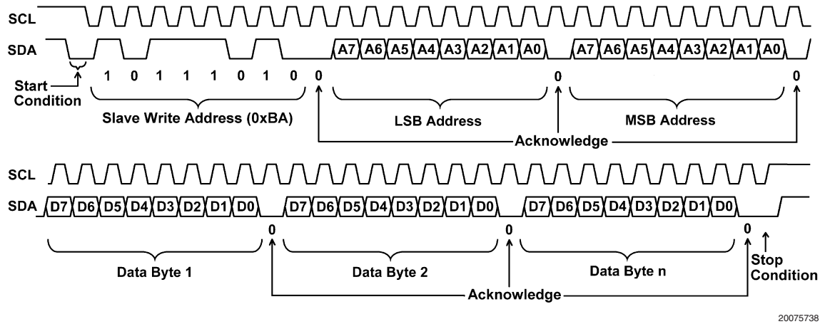
FIGURE 23. I²C Compatible Write Sequence
