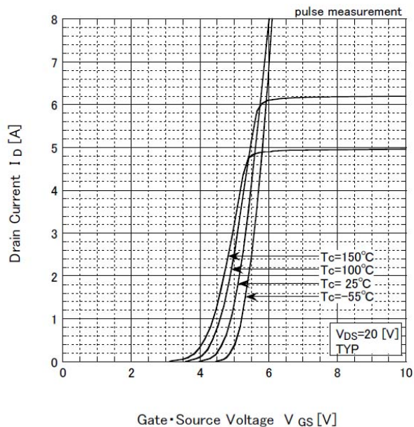
Transfer Characteristics
