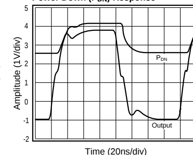
Power Down ( P_{DN} ) Response
