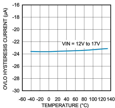
OVLO Hysteresis
