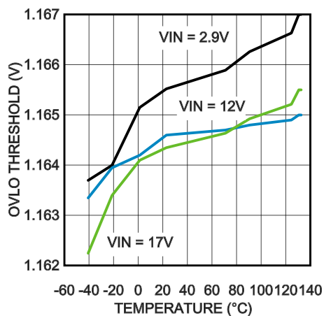
OVLO Threshold
