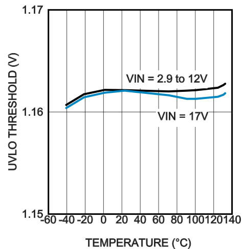
UVLO Threshold
