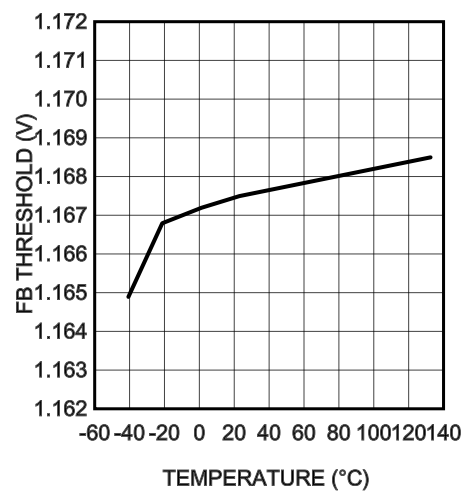
FB Threshold
