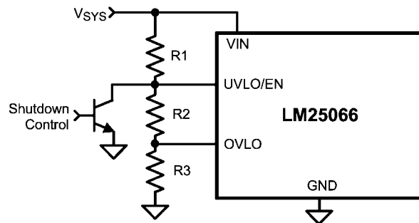
FIGURE 5. Shutdown Control
