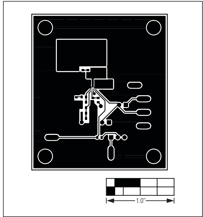
Figure 3. MAX15053 EV Kit Component PCB Layout—Component Side
