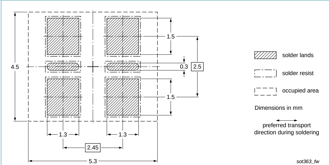
Fig 14. Wave soldering footprint PUMH15 (SOT363)
