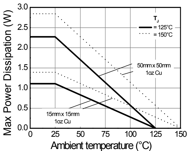
Derating Curve
