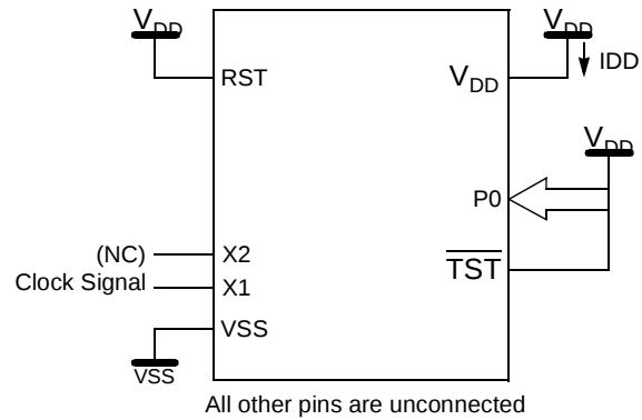
Figure 10. I_{DL} Test Condition, Idle Mode
