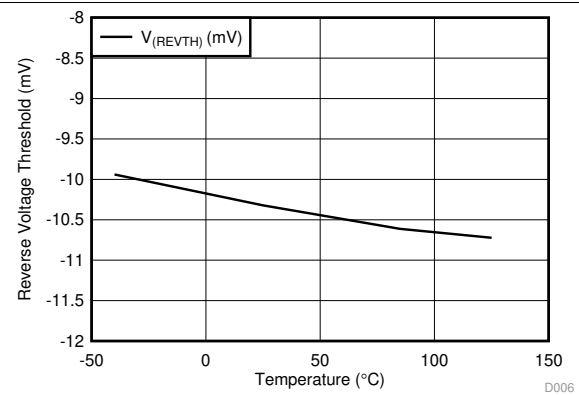
Figure 4. Reverse Voltage Threshold vs Temperature
