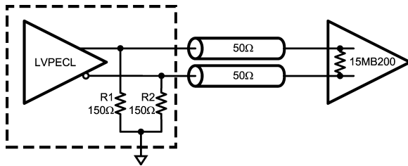
FIGURE 2. DC Coupled LVPECL to LVDS Interface
