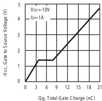
Figure 9. Gate Charge
