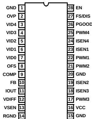
ISL6559CB (28 LEAD SOIC)
