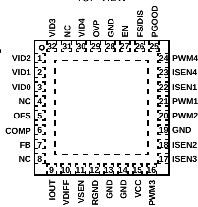
ISL6559CR (32 LEAD QFN)
